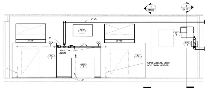
3 MECHANICAL SECTION 2 1/8\" = 1'-0"
